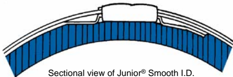
Sectional view of Junior® Smooth I.D. The "buckle nest" design significantly reduces leak paths.
