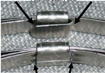
Buckle Nest Inside Diameter View Junior® Smooth ID Clamp
