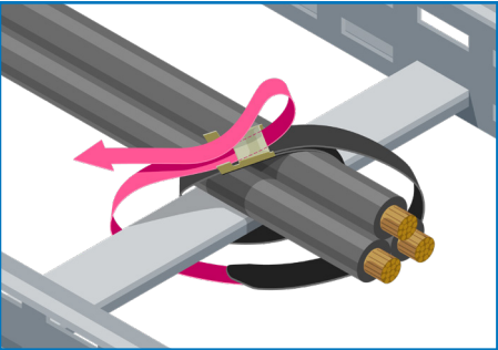
**Example of cross-wrap installation.
