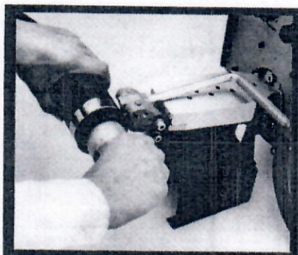
2. Depress toe end of foot pedal to tension clamp, keep toe end down. When pressure drops to holding pressure, roll clamp up.
