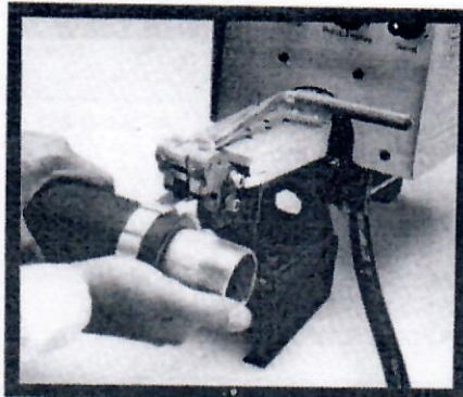
1. Insert clamp tail into nose of tool with buckle on top.
