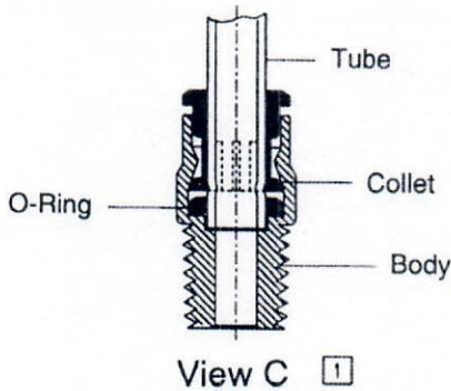
Push-In Fitting
