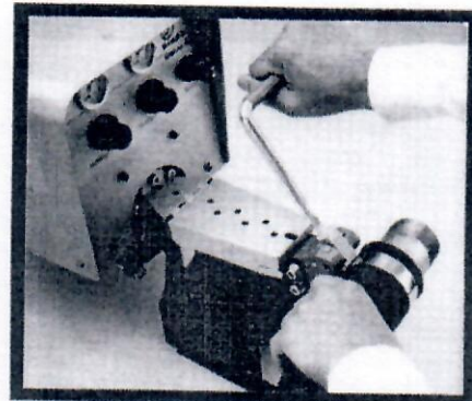
3. With clamp in full roll-up position, making sure shear hook is engaged onto buckle, pull cut-off lever to lock and complete clamp.
