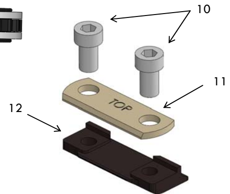
* J93099 Exploded View
